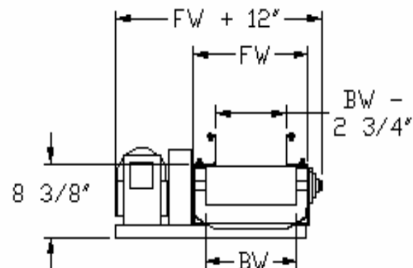
SIDE MOUNT DRIVE
